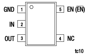
Figure 4. AAT3222 Pinout 5-Pin SOT23-5 (Top View)
