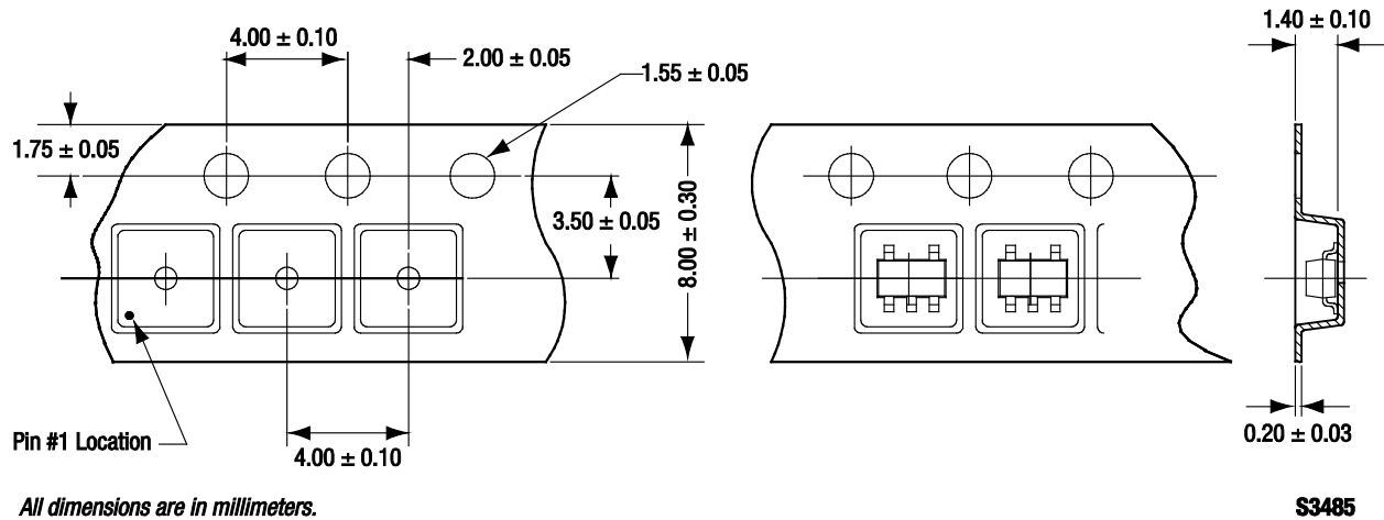
Figure 32. AAT3221/3222 Tape and Reel Dimensions (SOT23-5)
