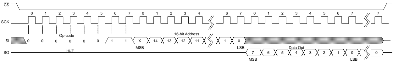
Figure 10. Memory Read
