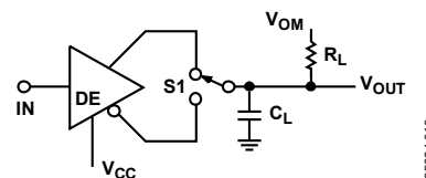
Figure 19. Driver Propagation Delay Test Circuit
