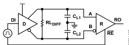
Figure 20. Driver/Receiver Propagation Delay Test Circuit
