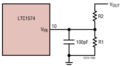
Figure 3. LTC1574 Adjustable Configuration
