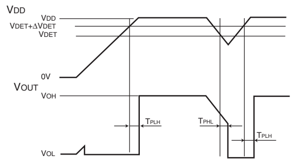
Timing waveform
