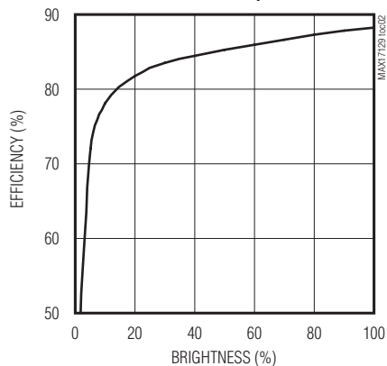
BOOST CONVERTER EFFICIENCY vs. BRIGHTNESS
