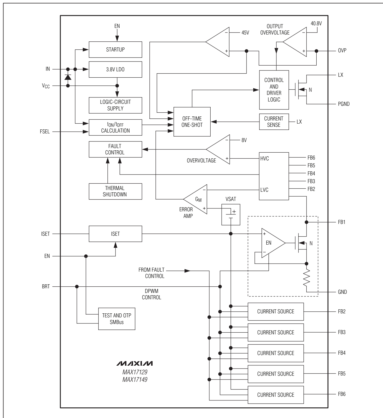
Figure 2. Functional Diagram
