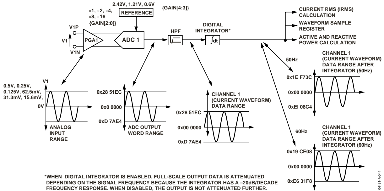
Figure 43. ADC and Signal Processing in Channel 1
