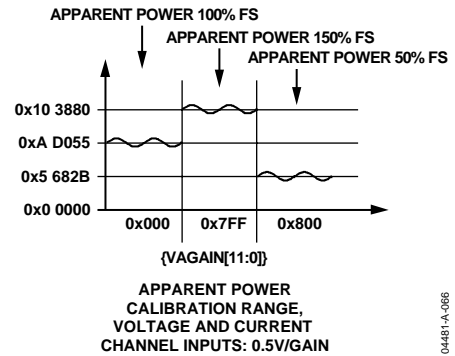
Figure 65. Apparent Power Calculation Output Range
