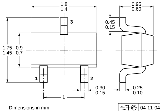
Fig 12. Package outline PDTC114EE (SOT416/SC-75)
