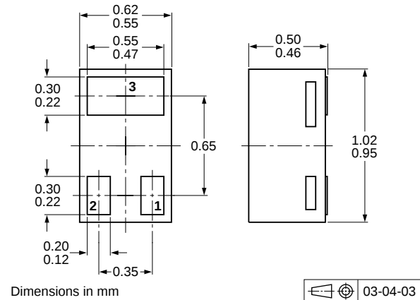
Fig 13. Package outline PDTC114EM (SOT883/SC-101)
