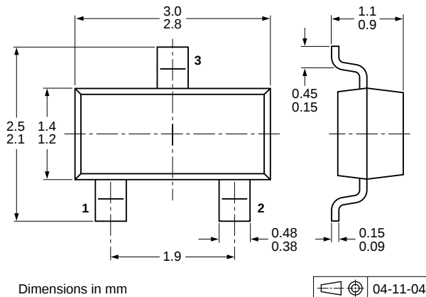
Fig 14. Package outline PDTC114ET (SOT23)
