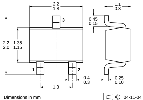
Fig 15. Package outline PDTC114EU (SOT323/SC-70)
