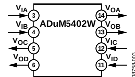
Figure 3. ADuM5402W
