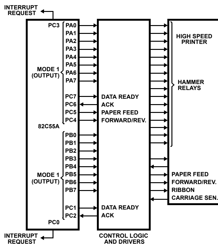
FIGURE 18. PRINTER INTERFACE
