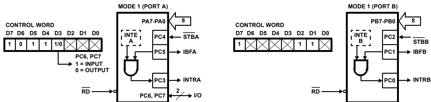
FIGURE 6. MODE 1 INPUT
