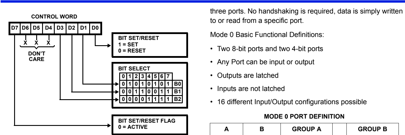
FIGURE 5. BIT SET/RESET FORMAT
