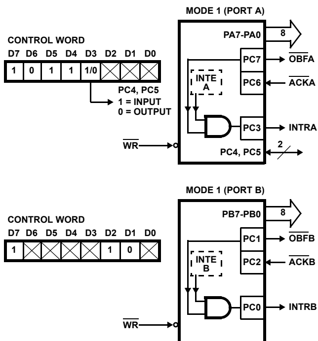
FIGURE 8. MODE 1 OUTPUT
