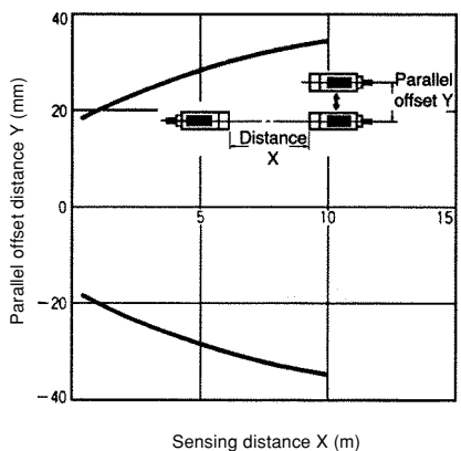
Through-beam Type E3L-2RC4 without aperture
