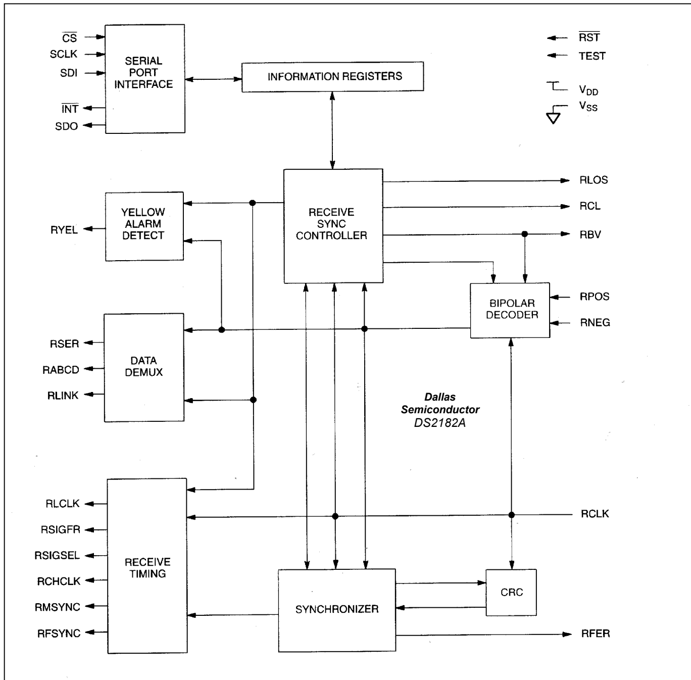
Figure 1. Block Diagram
