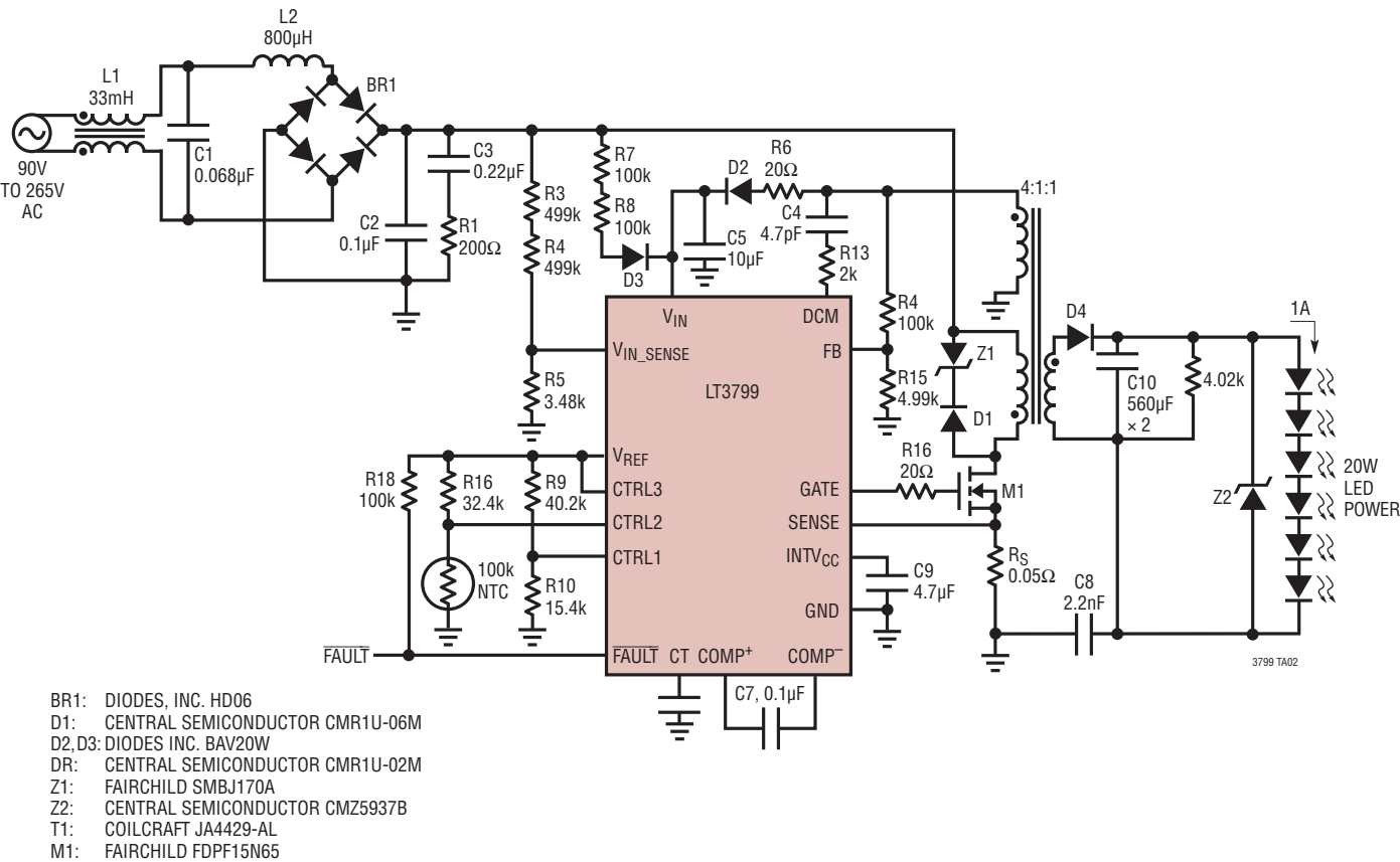
Universal TRIAC Dimmable 20W LED Driver
