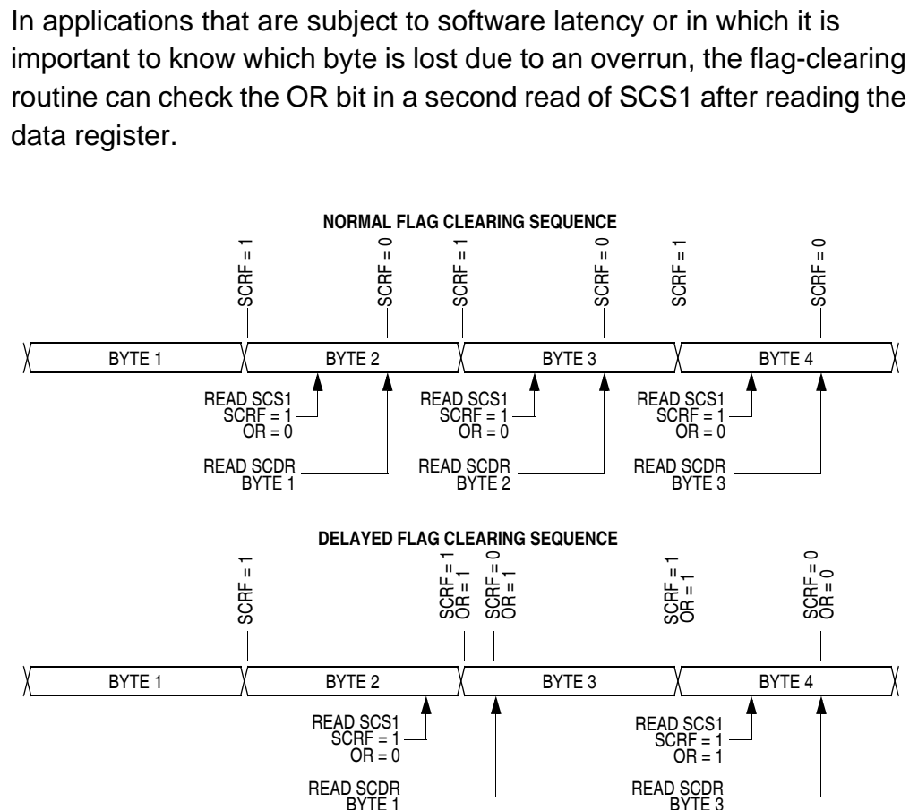
Figure 16-15. Flag Clearing Sequence
