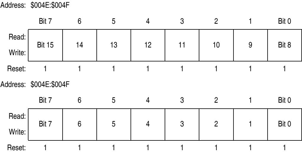
Figure 19-5. PIT Counter Modulo Registers (PMODH–PMODL)
