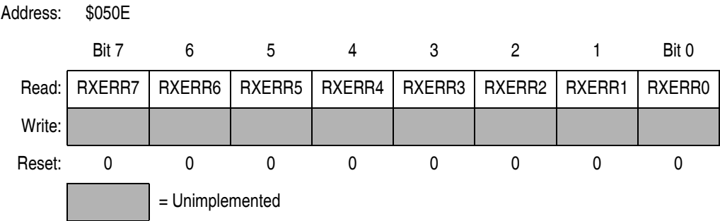
Figure 21-24. Receiver Error Counter (CRXERR)
