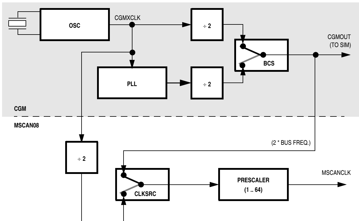
Figure 21-7. Clocking Scheme
