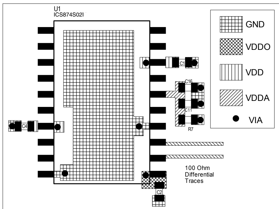
Figure 5B. PCB Board Layout for ICS874S02I
