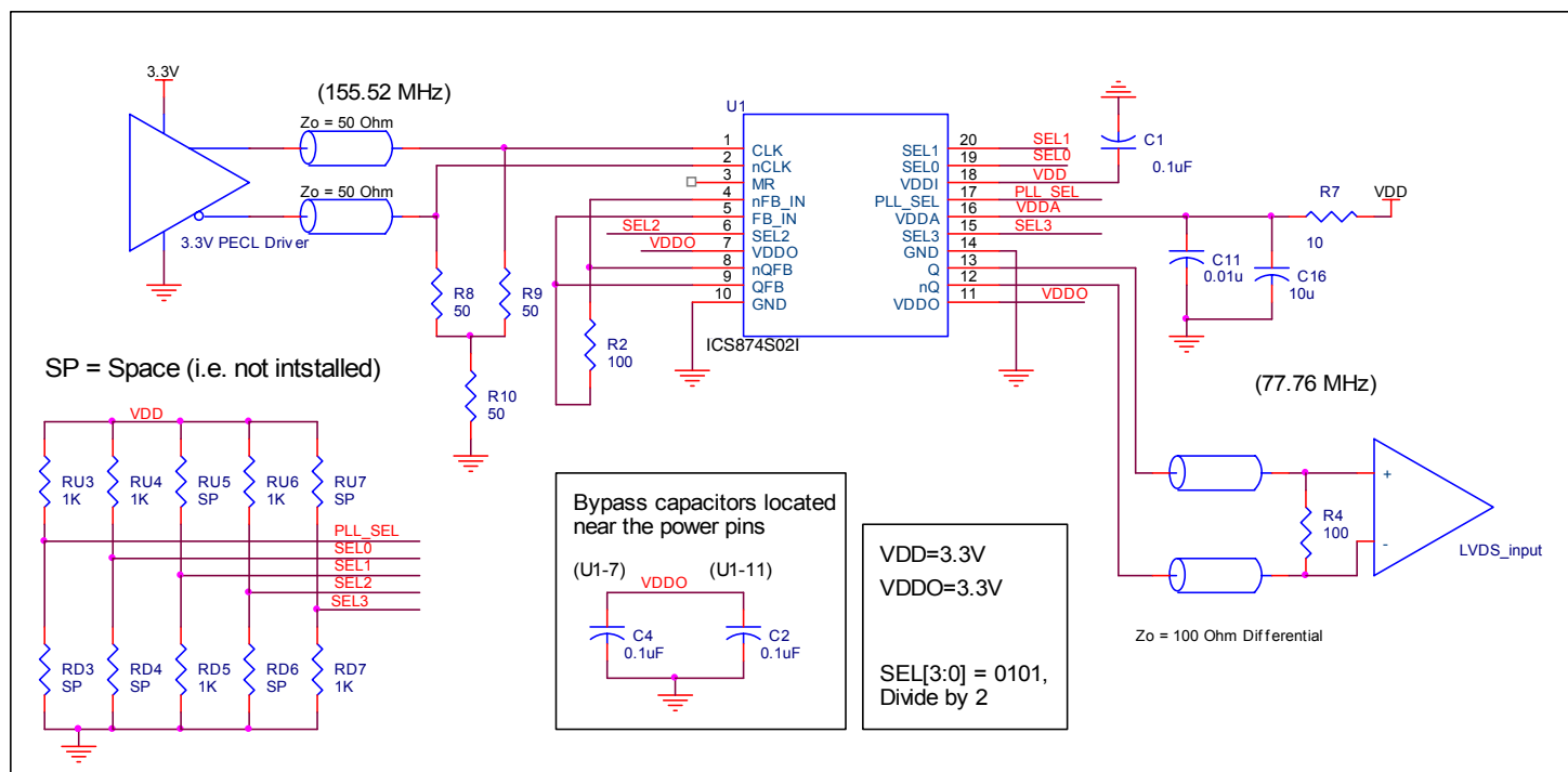
Figure 5A. ICS874S02I LVDS Zero Delay Buffer Schematic Example
