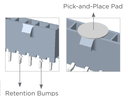
Retention Bumps
