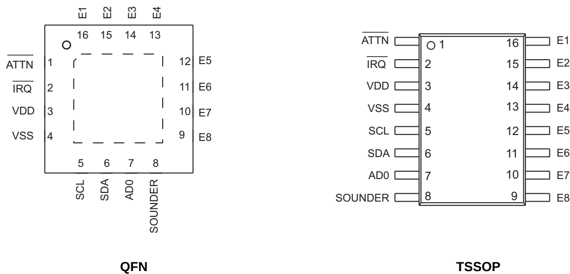
Figure 3. Package Pinouts
