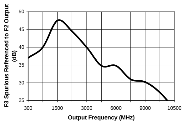
Spurious Response
