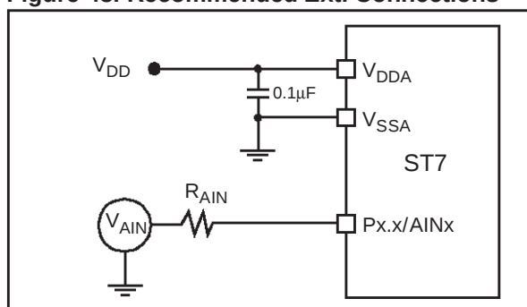
Figure 43. Recommended Ext. Connections
