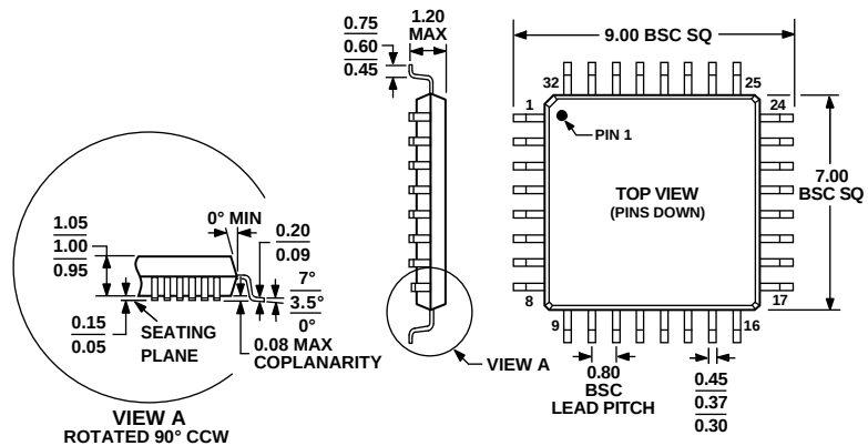
Figure 48. 32-Lead Thin Quad Flat Package [TQFP] (SU-32-2) Dimensions shown in millimeters
