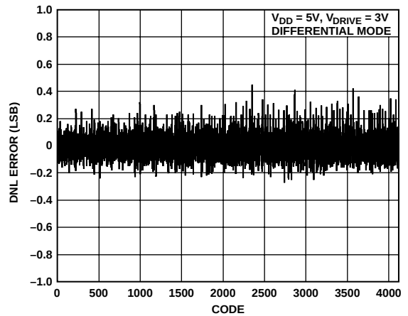
Figure 8. Typical DNL
