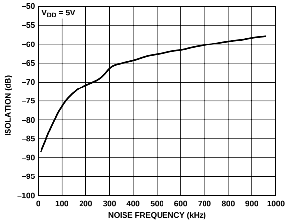
Figure 5. Channel-to-Channel Isolation
