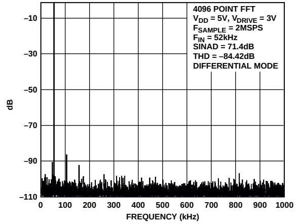
Figure 7. FFT
