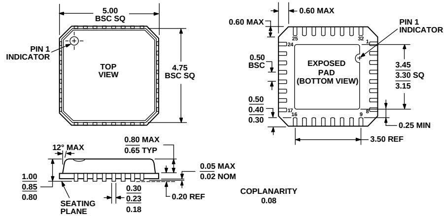
Figure 47. 32-Lead Frame Chip Scale Package [LFCSP] (CP-32-3) Dimensions shown in millimeters
