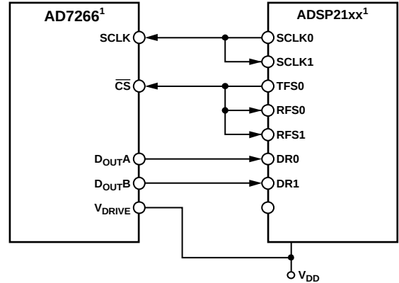
Figure 43. Interfacing the AD7266 to the ADSP218x
