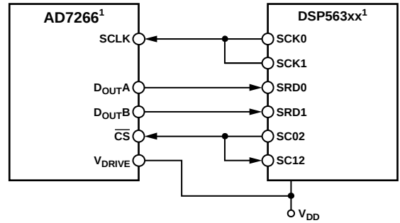
Figure 46. Interfacing the AD7266 to the DSP563xx
