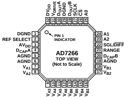
Figure 2. Pin Configuration (CP-32-3)
