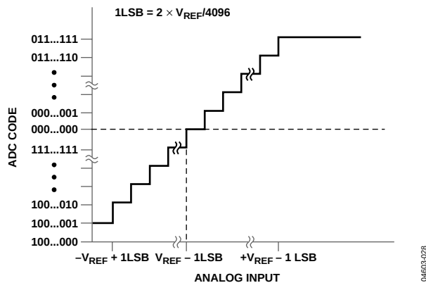
Figure 33. Twos Complement Transfer Characteristic with V_{REF} \pm V_{REF} Input Range
