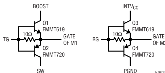
Figure 7. Optional External Gate Driver
