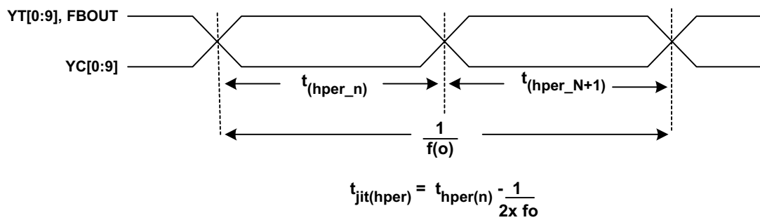
Figure 5. Half-Period Jitter
