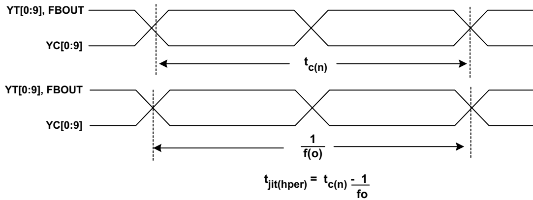
Figure 4. Period Jitter
