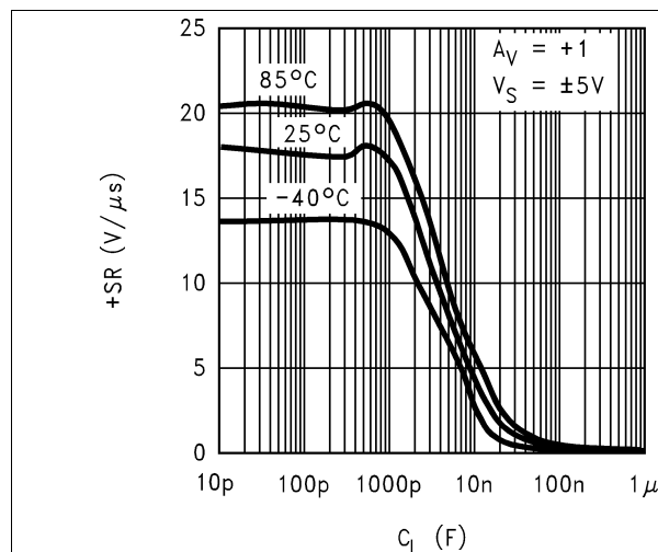
Figure 62. +SR vs. Capacitive Load
