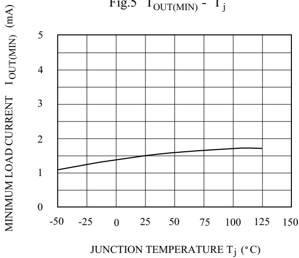
Fig.5 I_{OUT(MIN)} - T_j
