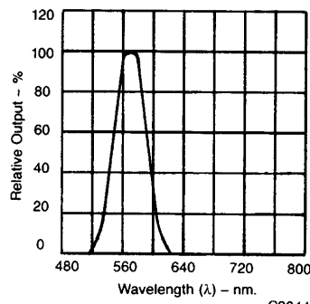
Fig. 2. Spectral Response
