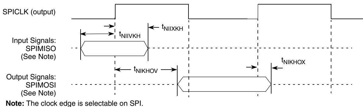
Figure 66. SPI AC Timing in Master Mode (Internal Clock) Diagram
