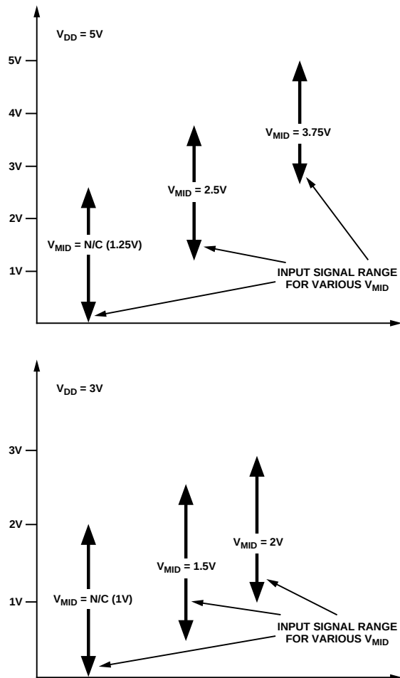
Figure 7. Analog Input Span Variation with V_{MID}
