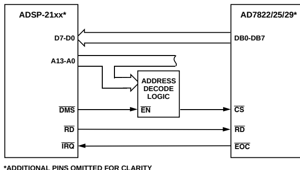
Figure 25. Interfacing to the ADSP-21xx
