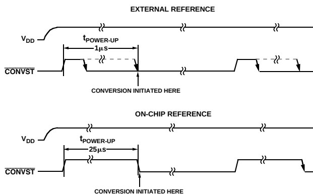
Figure 15. AD7829 Power-Up Time
