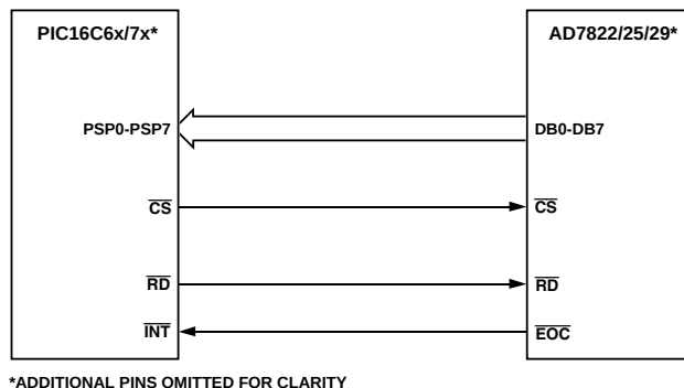
Figure 24. Interfacing to the PIC16C6x/7x
