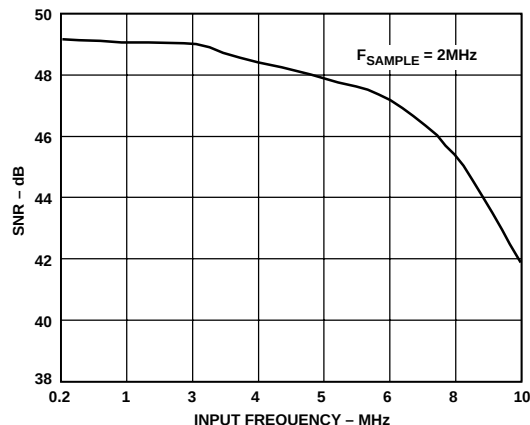
Figure 14. SNR vs. Input Frequency on the AD7825
