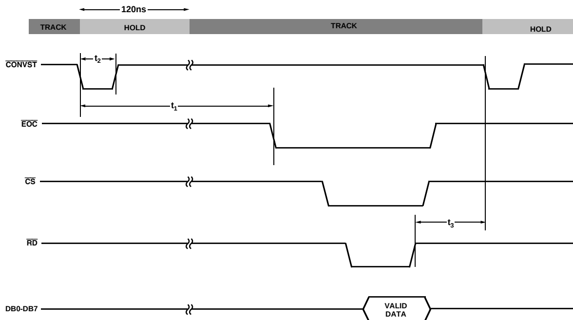
Figure 20. Mode 1 Operation
