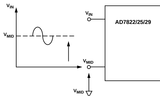
Figure 8. Removing Offsets Using V_{MID}
