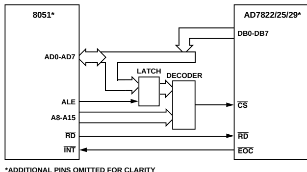
Figure 23. Interfacing to the 8051
