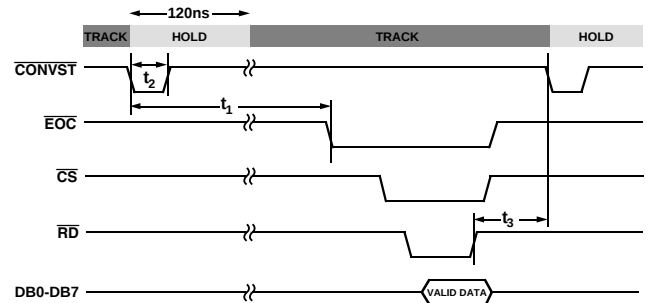
Figure 4. Track-and-Hold Timing
