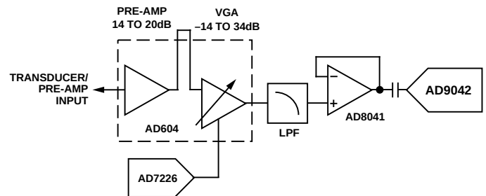
Figure 58. Using the AD9042 in Ultrasound Applications
