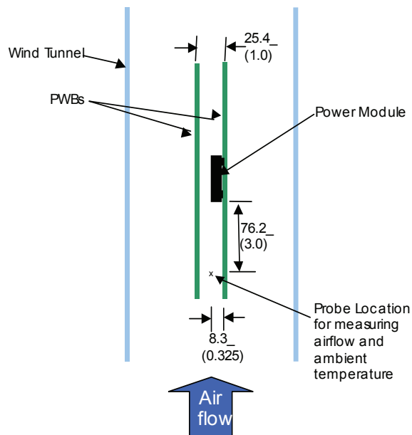
Figure 32. Thermal Test Set-up.
