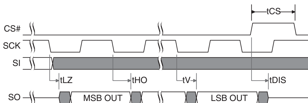
Figure 30. SPI Single Bit Output Timing
