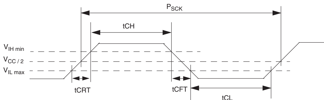
Figure 28. Clock Timing
