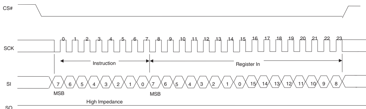
Figure 94. ASPP Command
