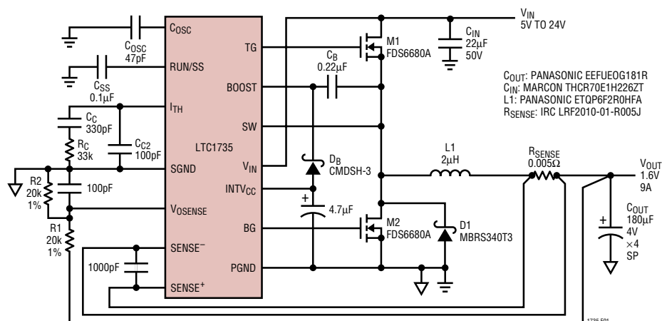
Figure 1. High Efficiency Step-Down Converter
