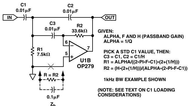
Figure 15. Two-Pole, High Pass Multiple Feedback Filters
