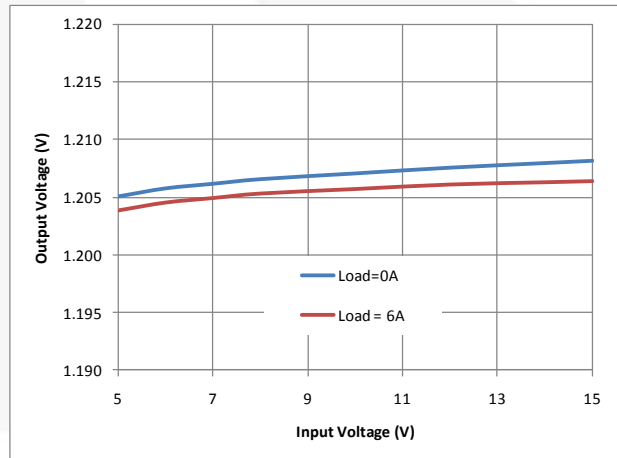
Figure 14. Line Regulation
