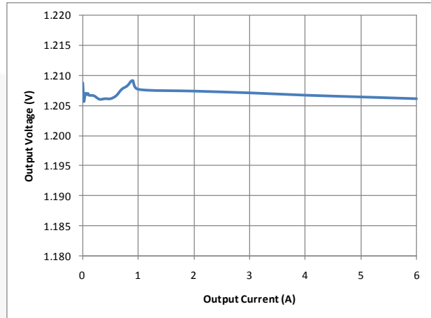
Figure 12. Load Regulation
