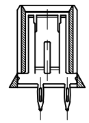
SECTION: W-W (4.00)
