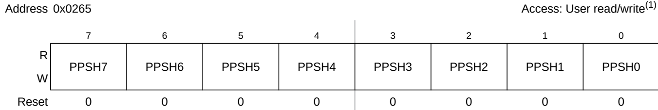
Figure 19-56. Port H Polarity Select Register (PPSH)
