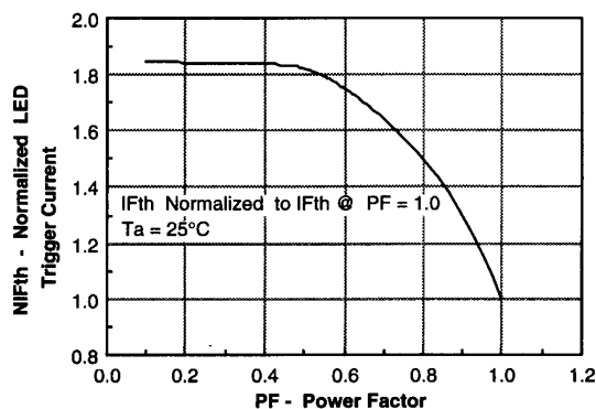
Figure 8. Normalized LED trigger current
