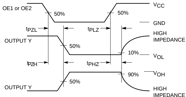
Figure 4. Switching Waveform
