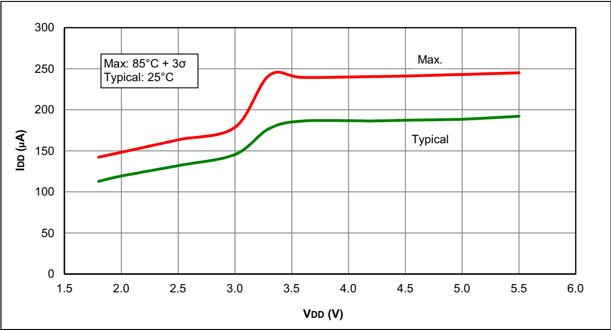
FIGURE 31-22: I_{DD} , MFINTOSC, F_{osc} = 500\text{ kHz} , PIC16F1938/9 ONLY
