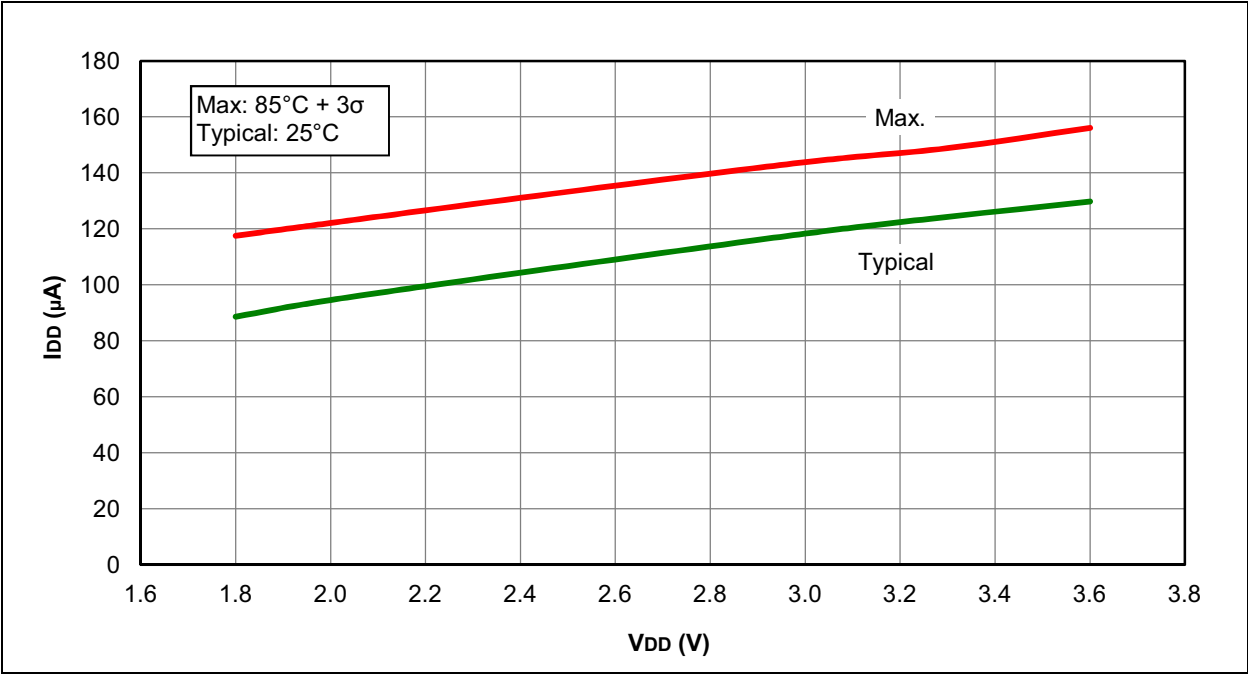
FIGURE 31-21: I_{DD} , MFINTOSC, F_{osc} = 500\text{ kHz} , PIC16LF1938/9 ONLY
