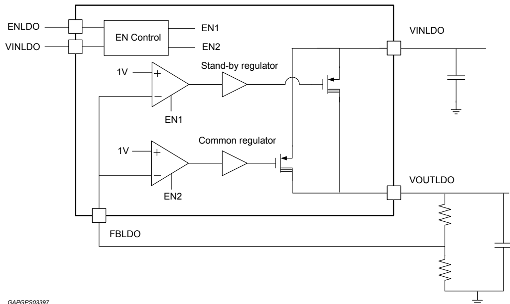
Figure 7. LDO diagram
