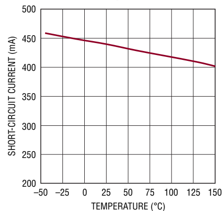
LD02, LD03, LD04 Short-Circuit Current vs Temperature
