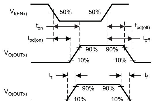
Figure 2. Timing and Internal Voltage Regulator Transition Waveforms
