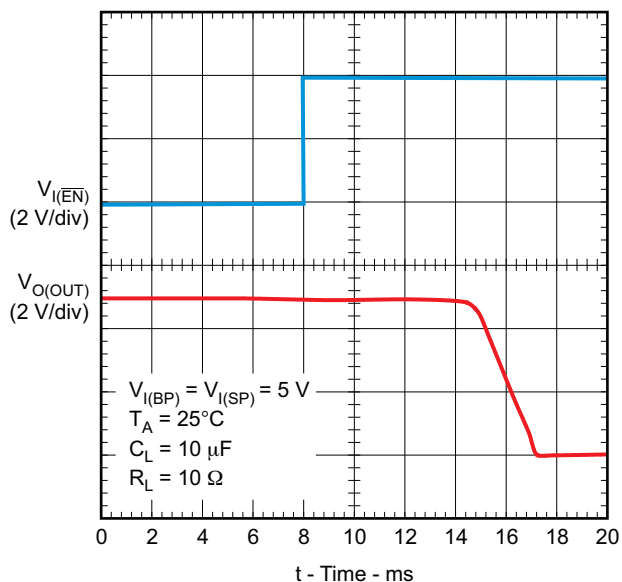
Figure 6. Turnoff Delay and Fall Time (SP Switch)
