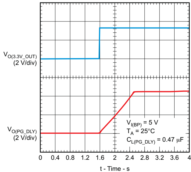
Figure 9. PG_DLY Rise Time With a 0.47-μF Capacitor
