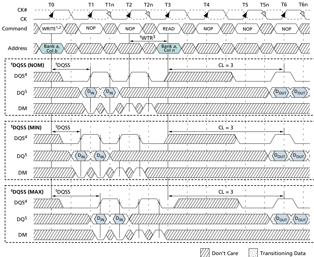
Figure 40: WRITE-to-READ – Interrupting
