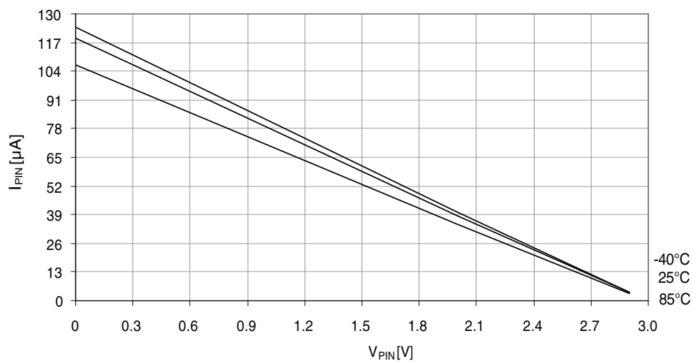
Figure 37-21. I/O pin pull-up resistor current vs. input voltage. V_{CC} = 3.0V .
