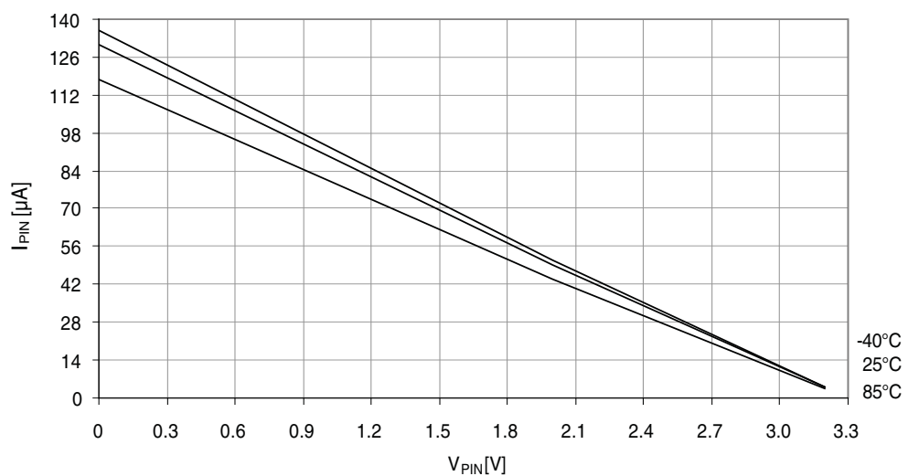
Figure 37-22. I/O pin pull-up resistor current vs. input voltage. V_{CC} = 3.3V .
