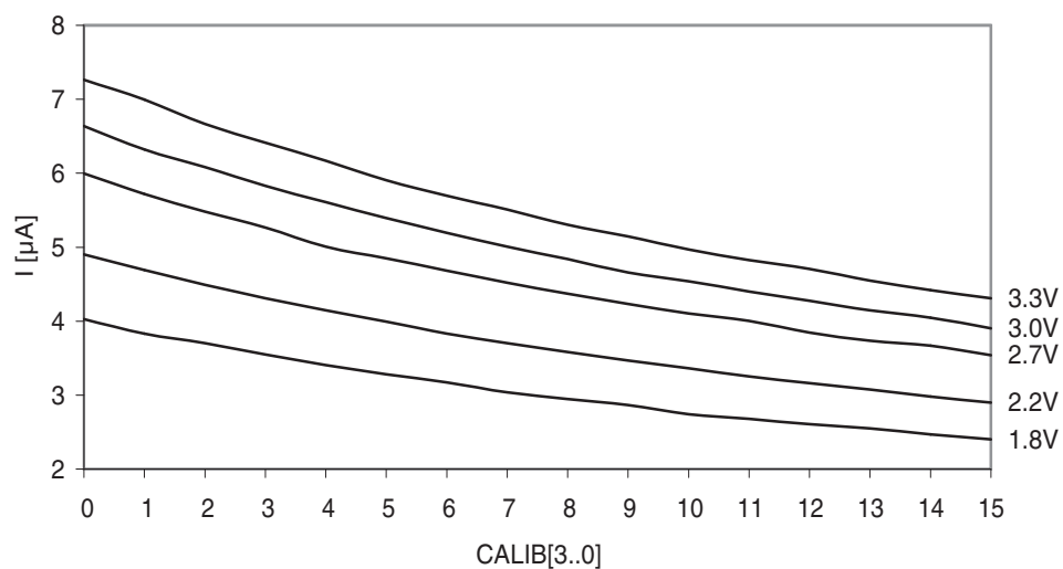
Figure 37-55. Analog comparator current source vs. calibration value. Temperature = 25°C.
