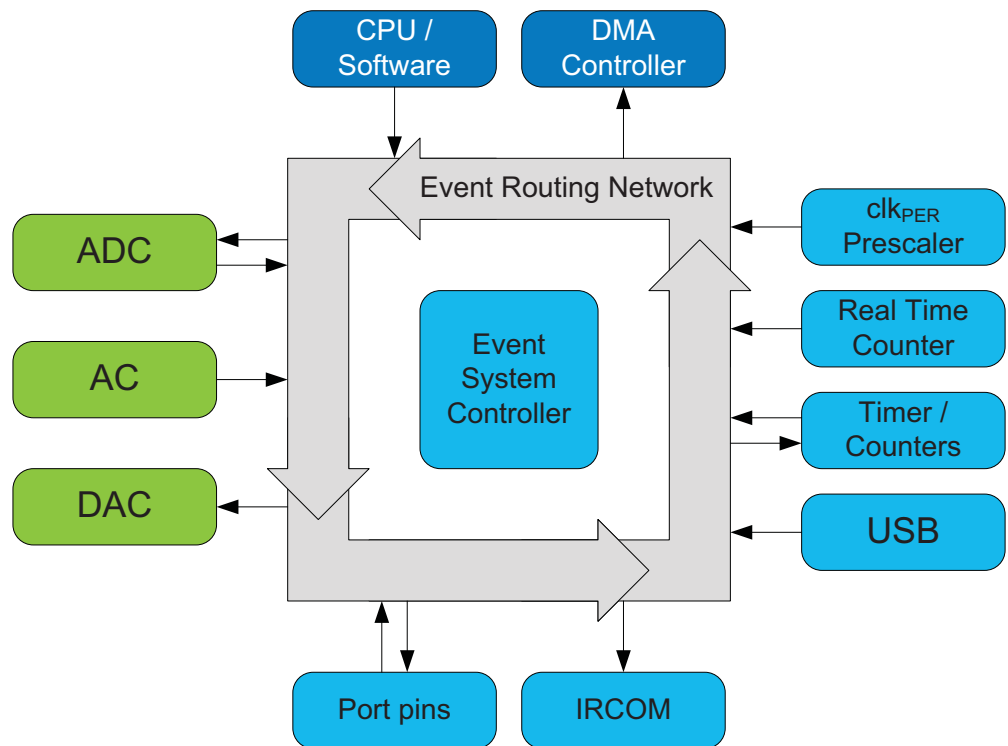
Figure 9-1. Event system overview and connected peripherals.
