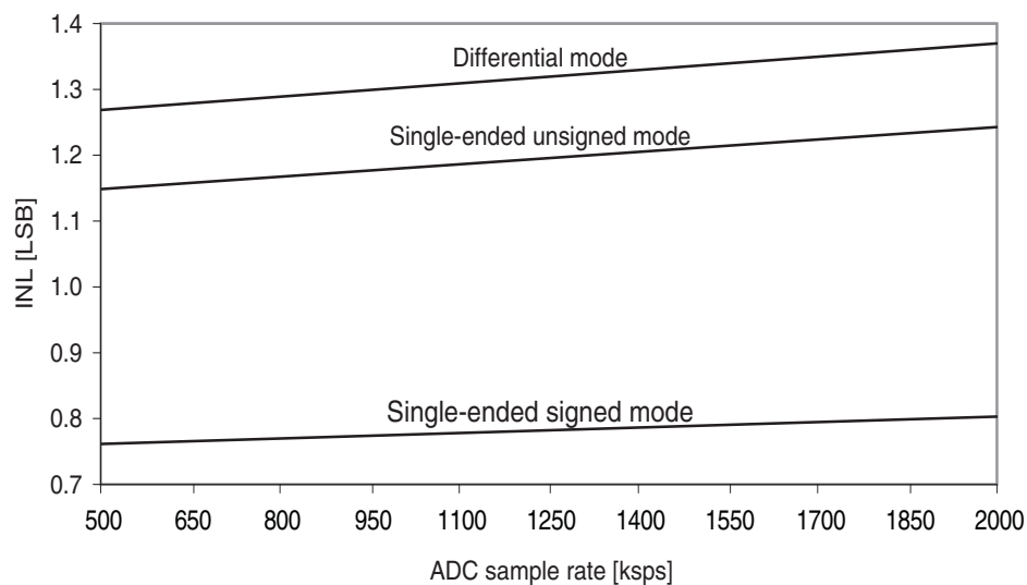
Figure 37-36. INL error vs. sample rate. T = 25^{\circ}\text{C} , V_{CC} = 3.6\text{V} , V_{REF} = 3.0\text{V} external.
