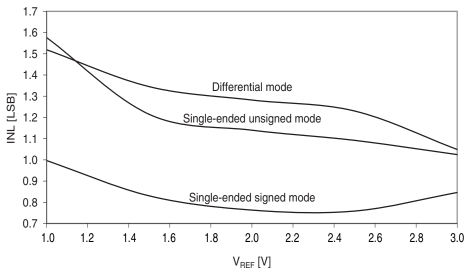
Figure 37-35. INL error vs. external V_{REF} . T = 25^{\circ}\text{C} , V_{CC} = 3.6\text{V} , external reference.
