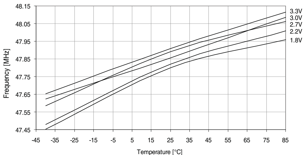
Figure 37-79. 48MHz internal oscillator frequency vs. temperature.
