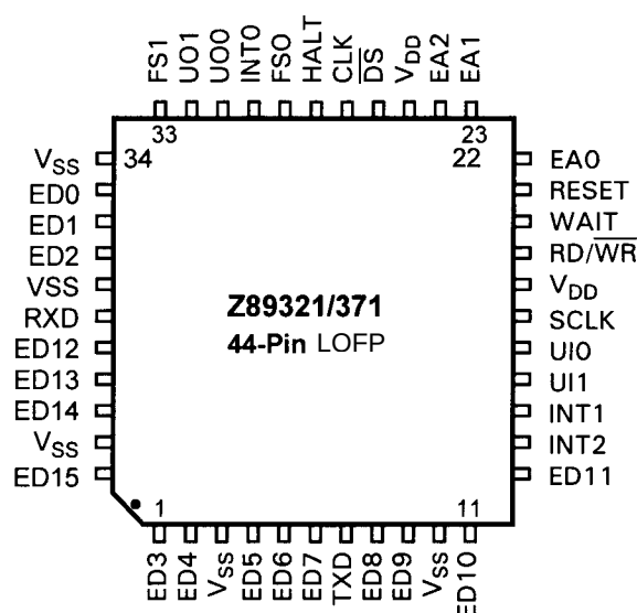
Figure 5. Z89321/371 44-Pin LOFP Pin Assignments
