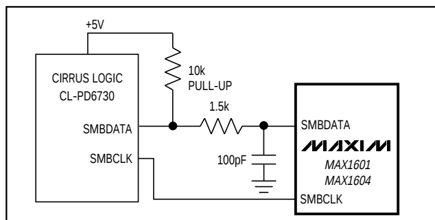
Figure 6. Application with Cirrus Logic Interface
