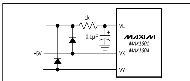
Figure 5. Powering from Either VX or VY
