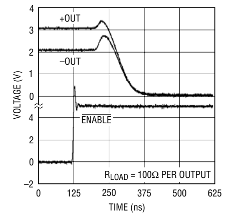
Turn-Off Time
