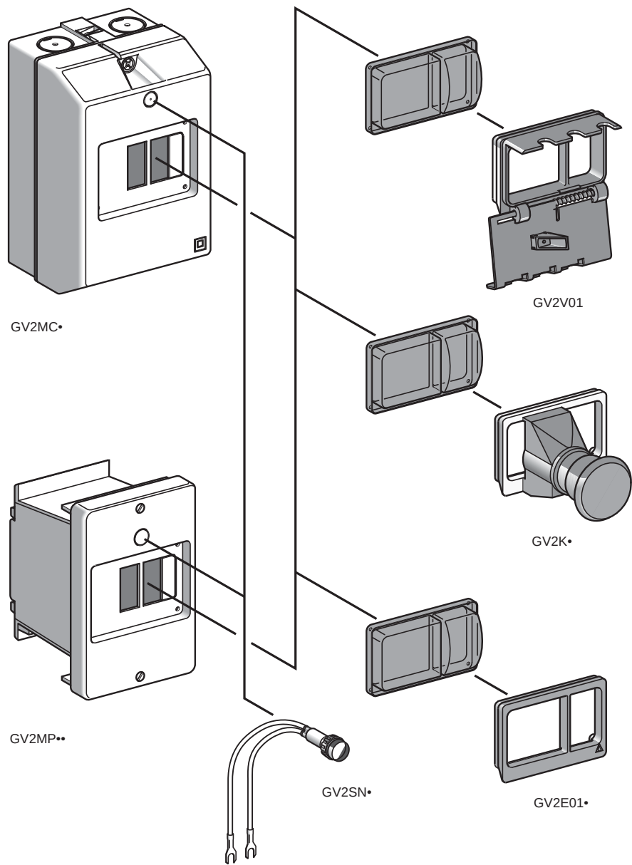
Figure 4: GV2M Enclosures
