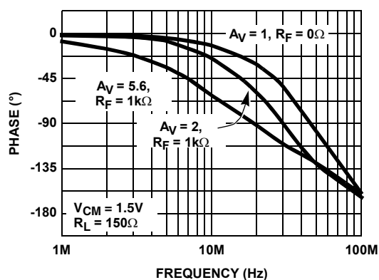
FIGURE 2. NON-INVERTING FREQUENCY RESPONSE (PHASE)
