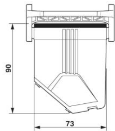
Dimensioned drawing
