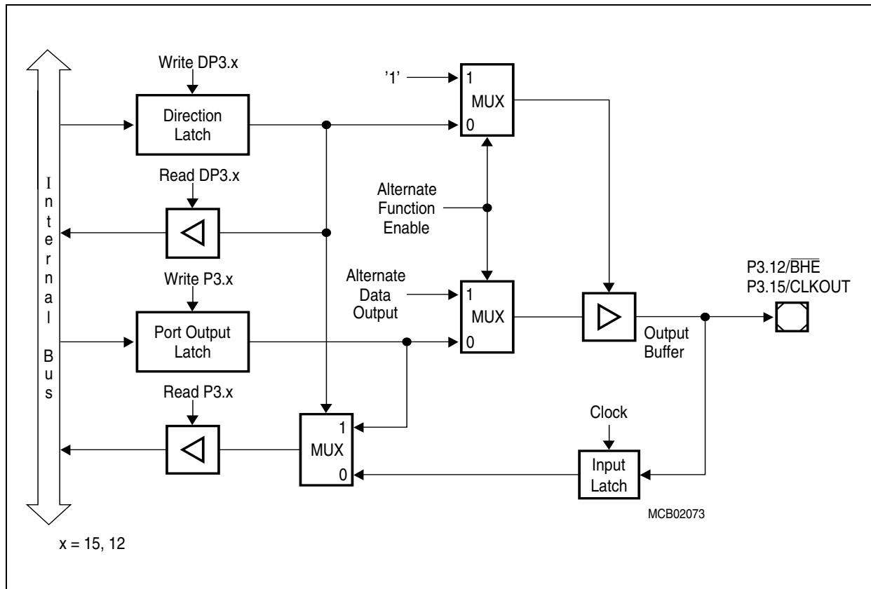
Figure 37 Block Diagram of Pins P3.15 (CLKOUT) and P3.12 ( \overline{\text{BHE}} / \overline{\text{WRH}} )
