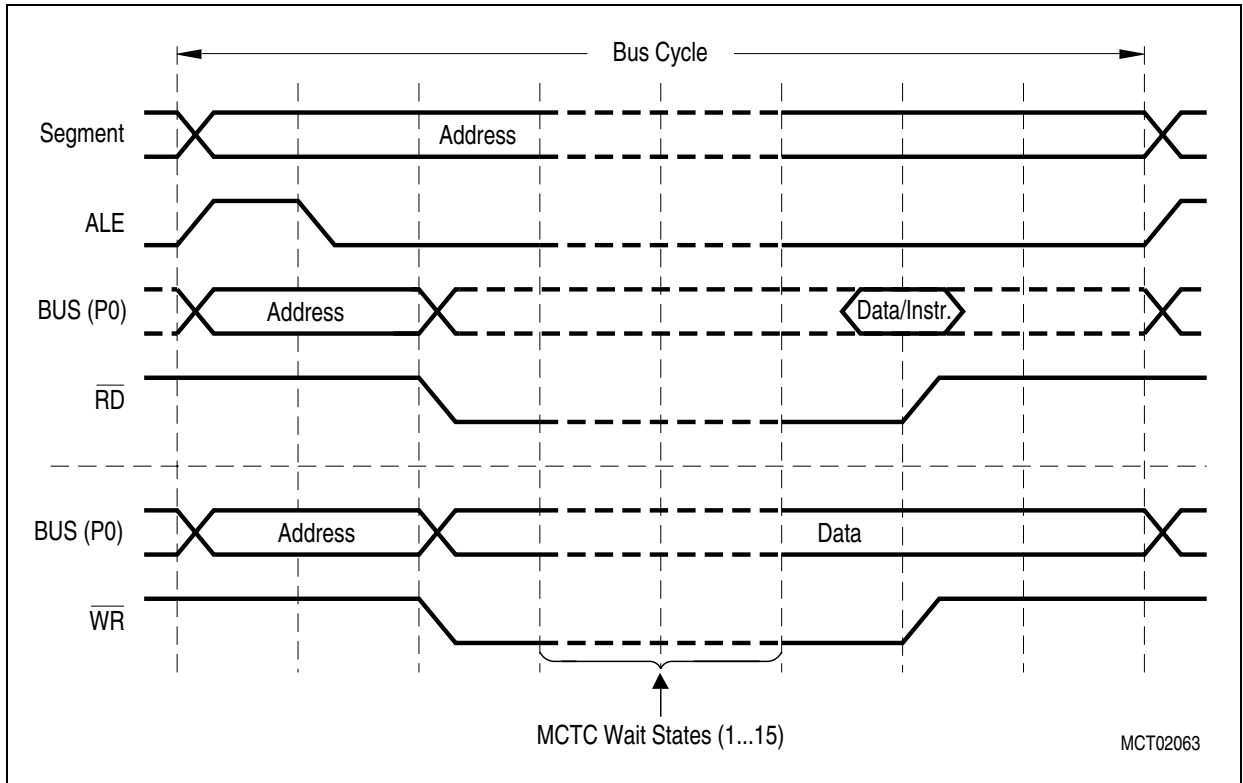
Figure 50 Memory Cycle Time
