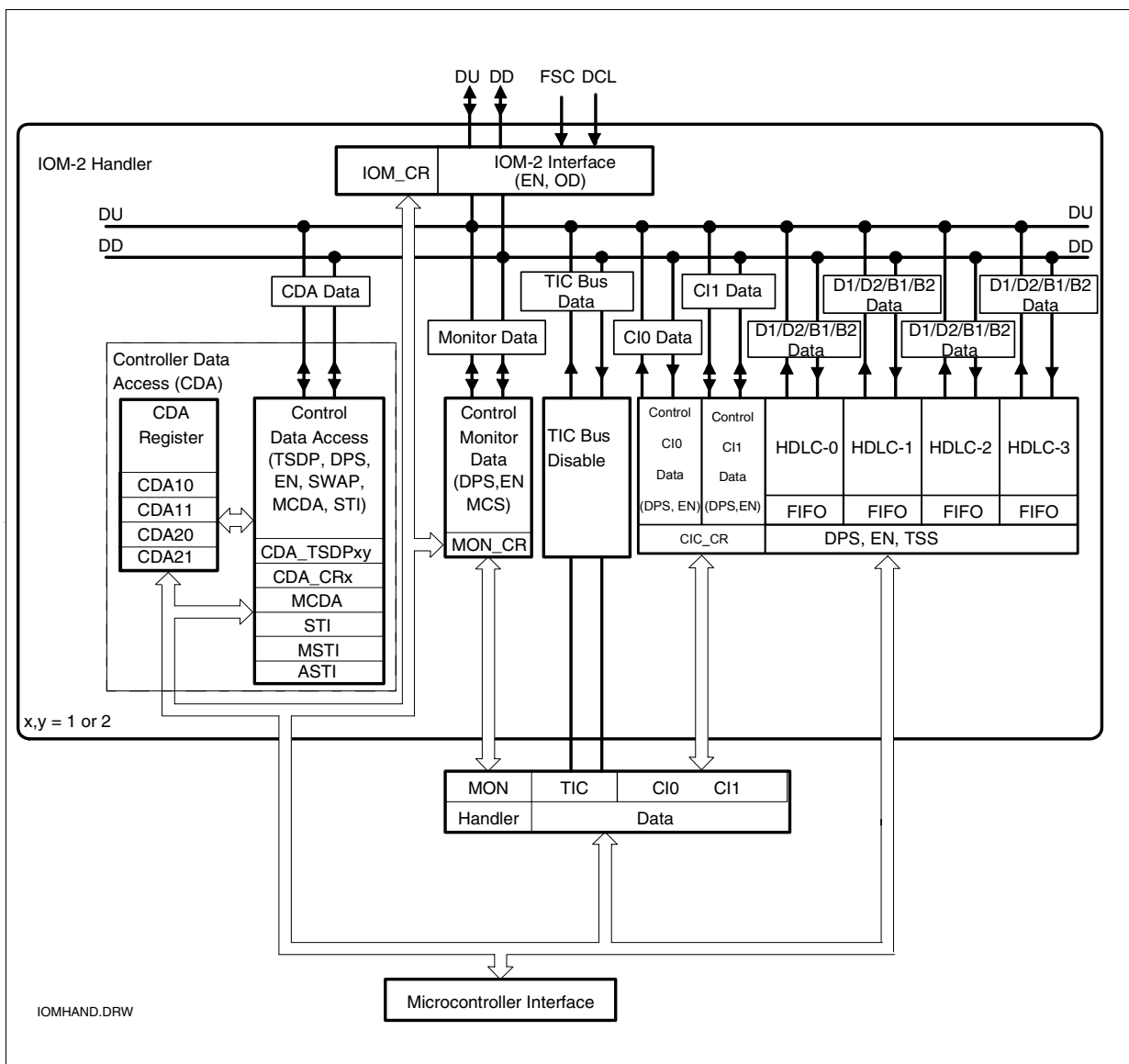
Figure 112 Architecture of the IOM-2 Handler
