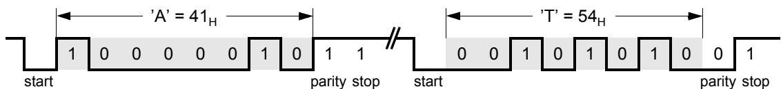
Figure 91 Two-Byte Serial Frames with ASCII 'AT'
