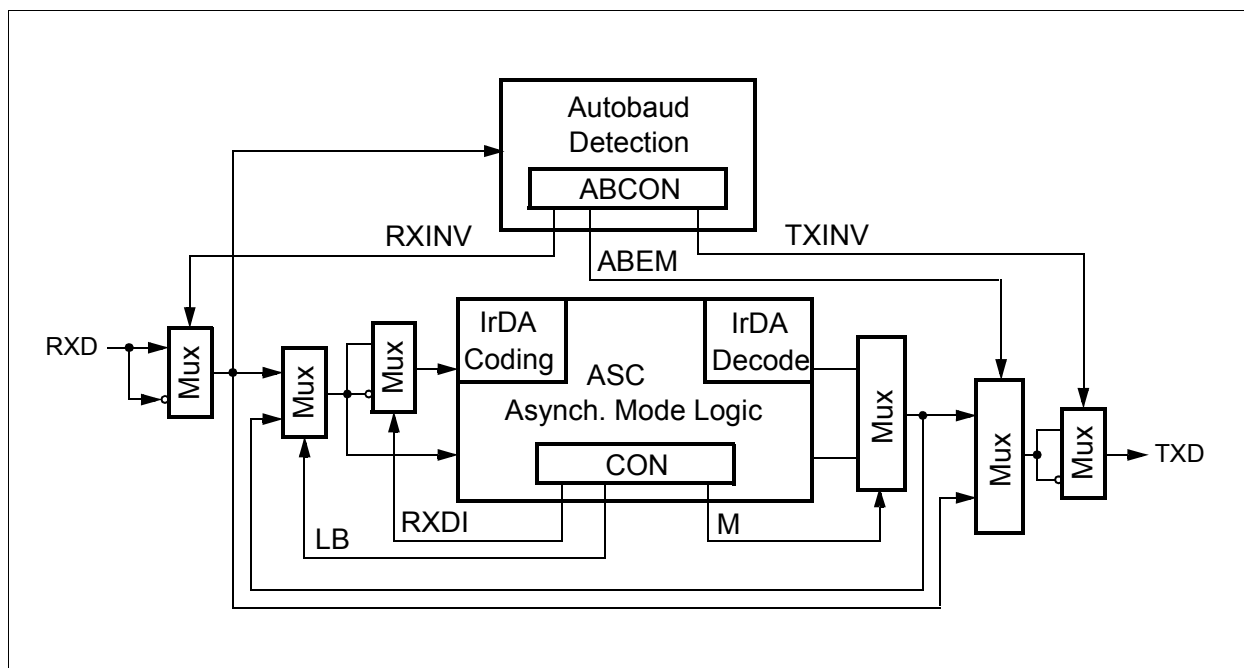
Figure 84 RXD/TXD Data Path in Asynchronous Modes (ASC)
