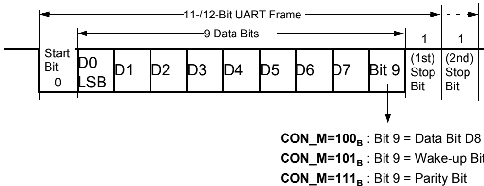
Figure 81 Asynchronous 9-Bit Frames
