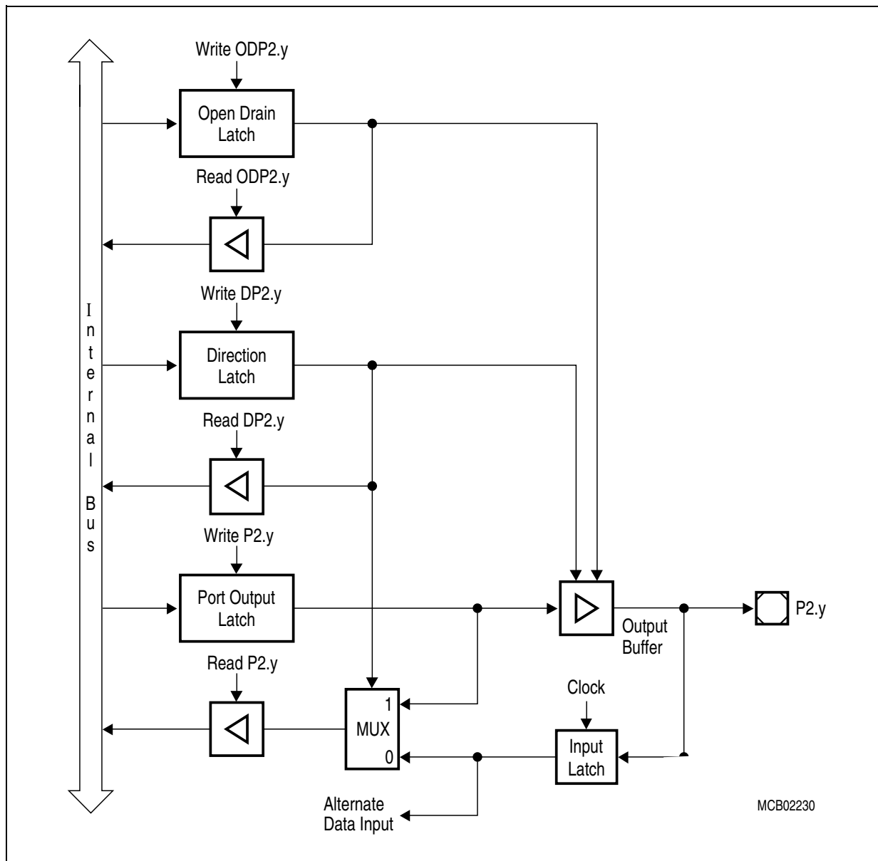
Figure 34 Block Diagram of a Port 2 Pin (y = 7...0)
