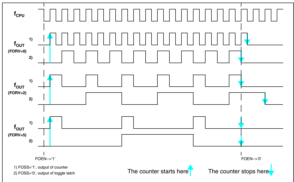
Figure 144 Signal Waveforms
