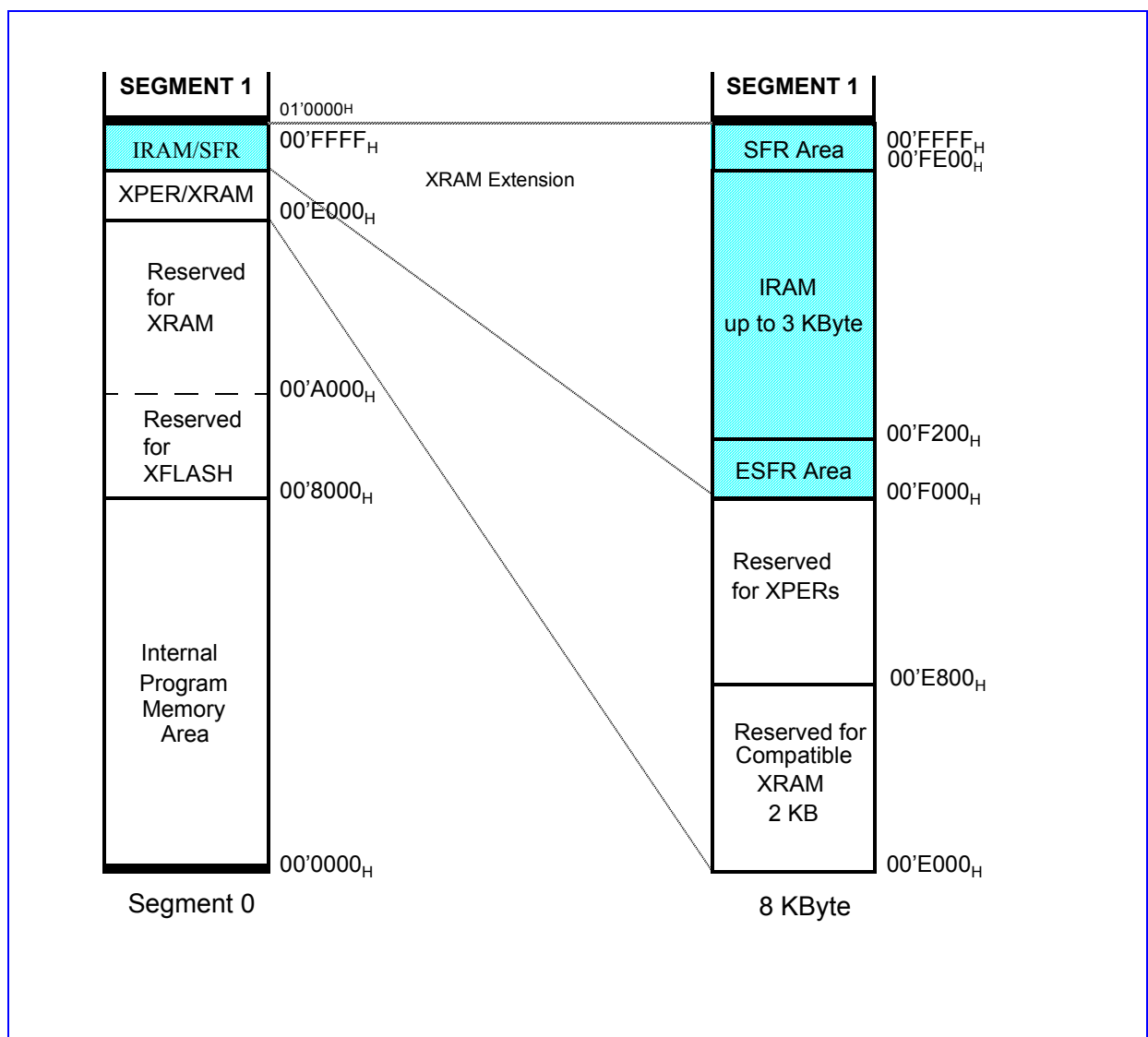
Figure 8 Memory Areas and Address Space
