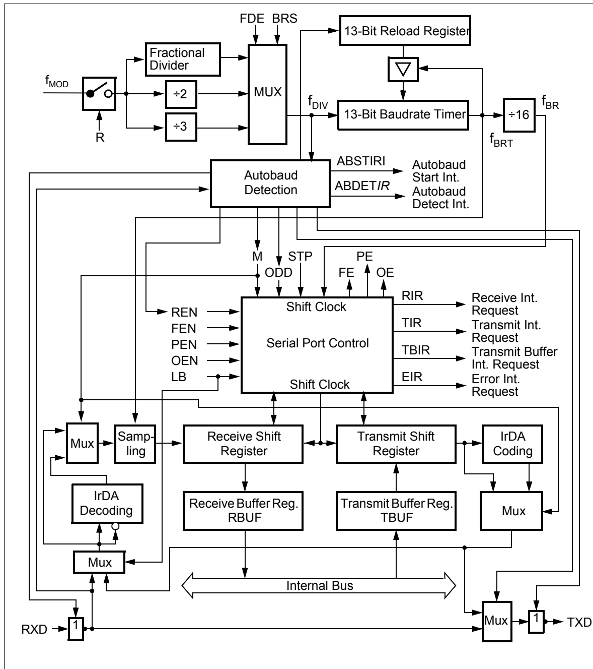
Figure 79 Asynchronous Mode of Serial Channel ASC
