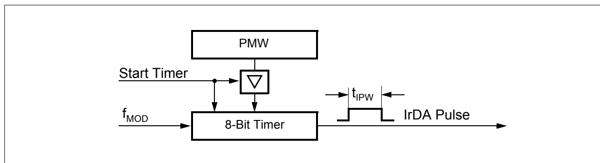
Figure 83 Fixed IrDA Pulse Generation
