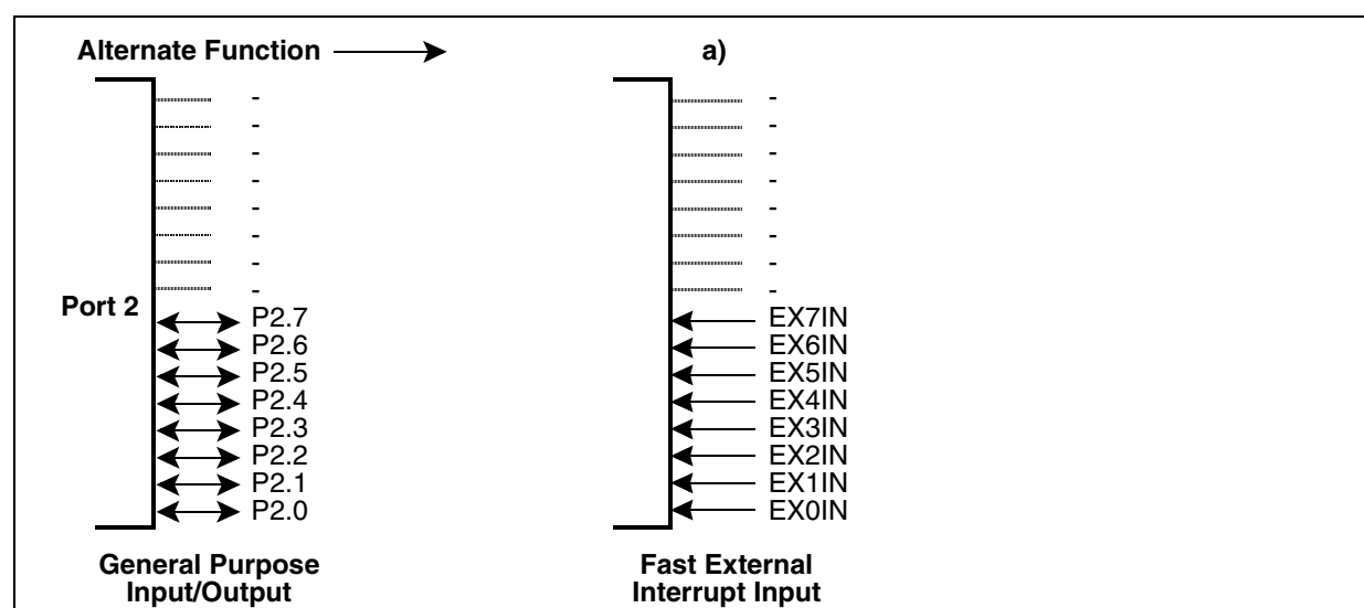
Figure 33 Port 2 I/O and Alternate Functions
