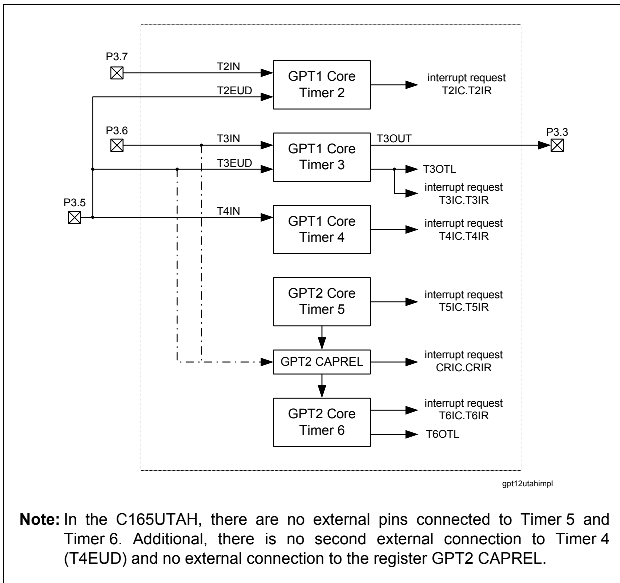
Figure 58 GPT module external pins
