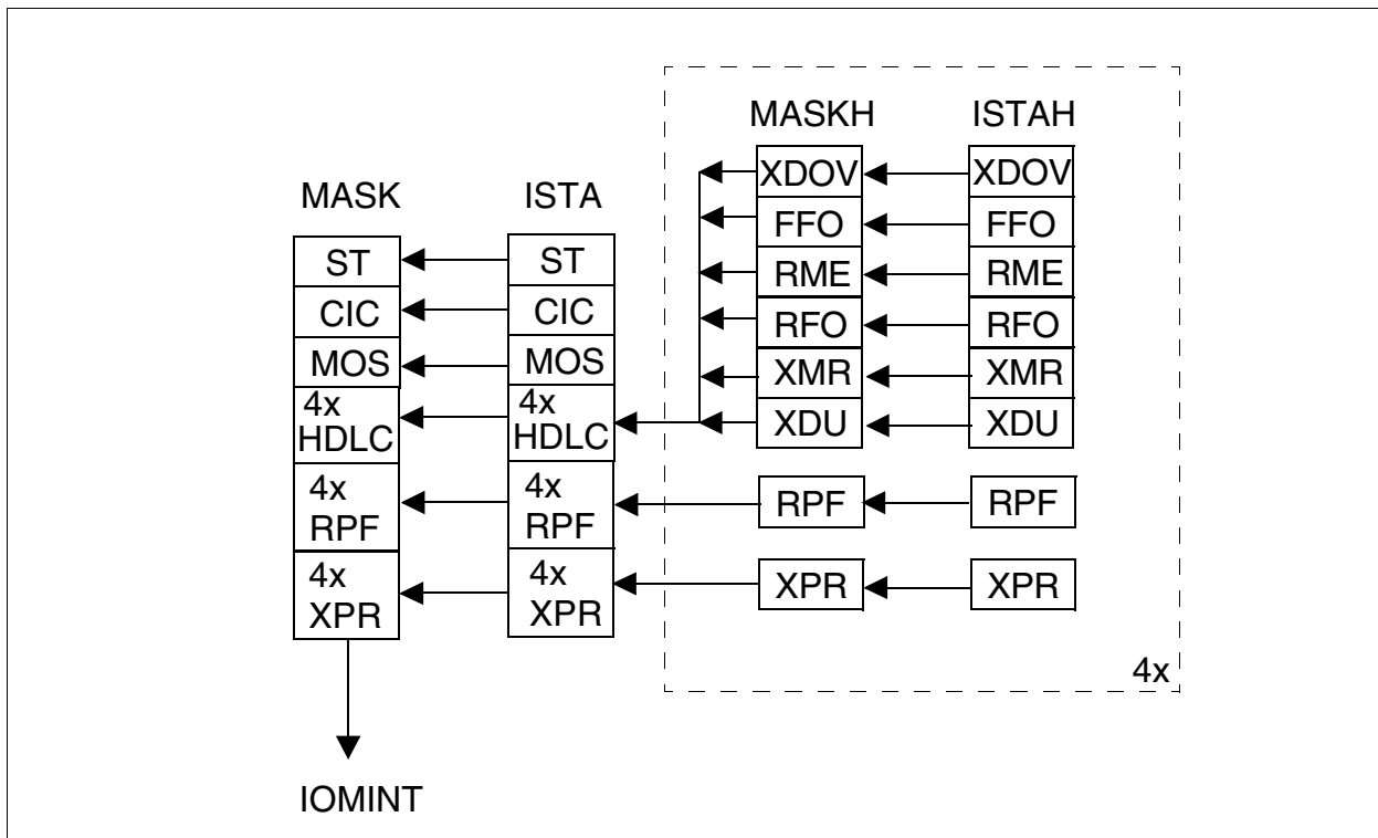
Figure 132 Interrupt Status Registers of the HDLC Controller
